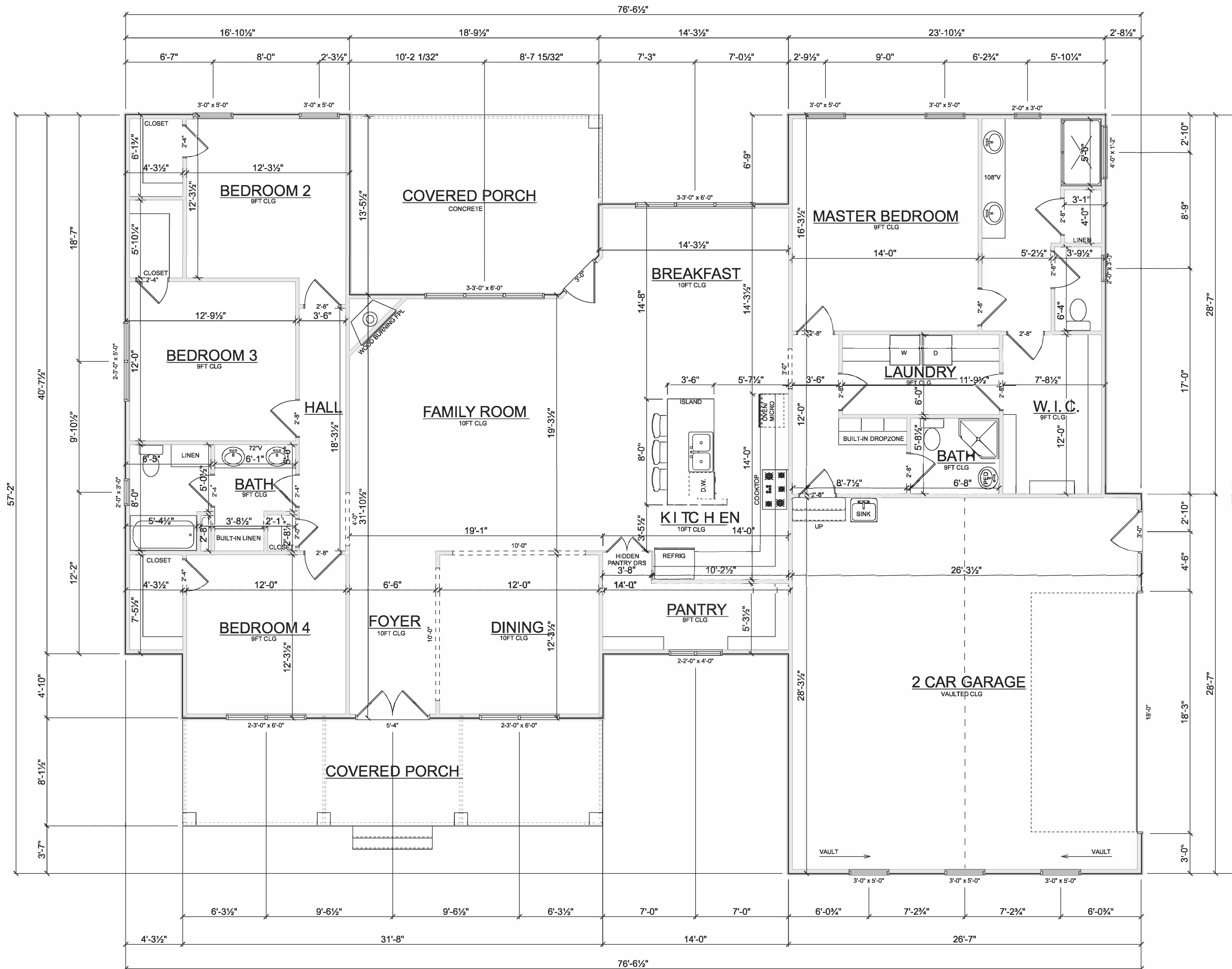
MAIN FLOOR SCALE: 1/4" = 1'-0"
