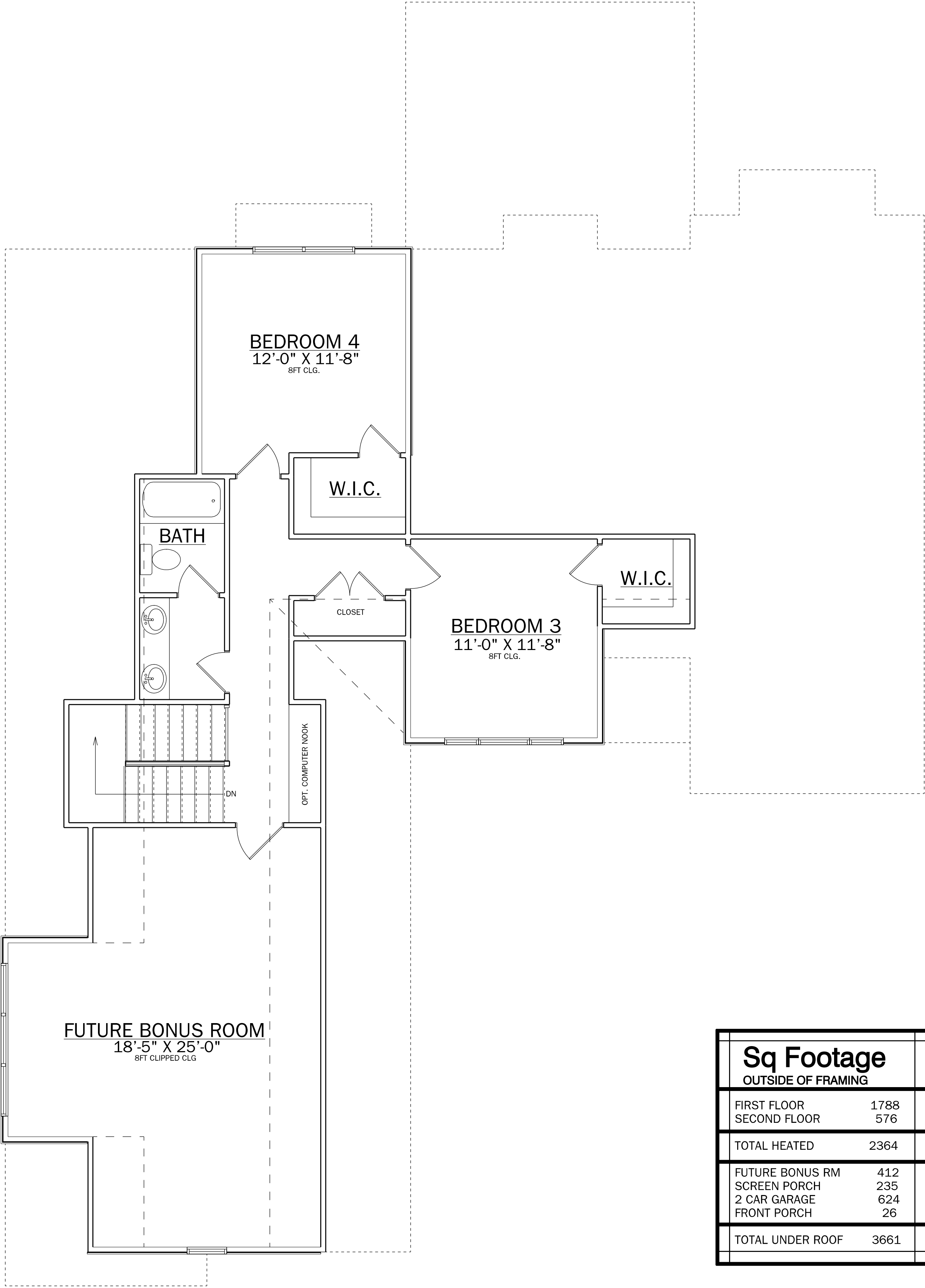
SECOND FLOOR
