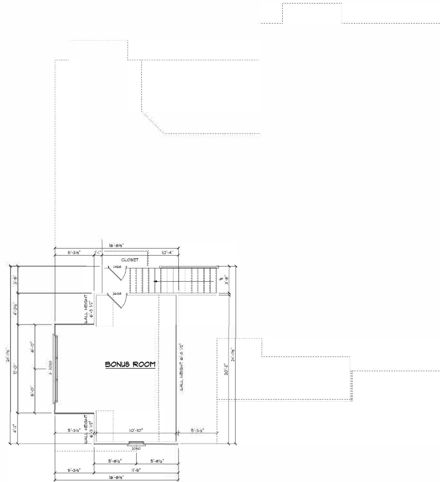
SECOND FLOOR WALLS SCALE: 1/4" = 1'-0"
