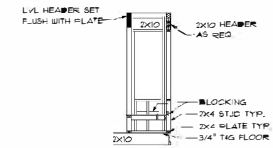
WINDOW SEAT FRAMING DETAIL
