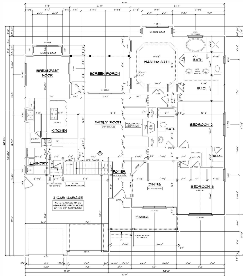
FIRST FLOOR WALLS SCALE: 1/4" = 1'-0"
