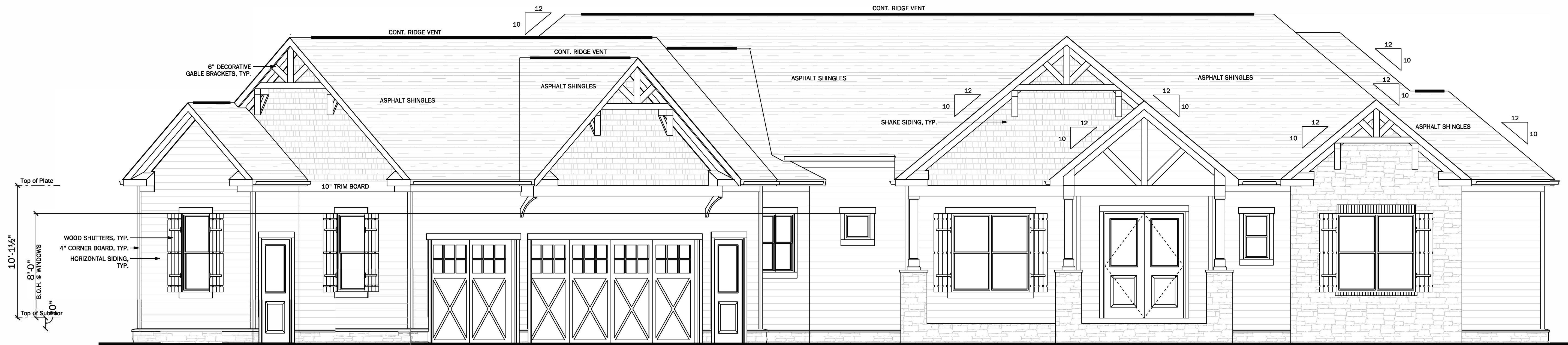
FRONT 12-27-17 SCALE: 1/4" = 1'-0"
