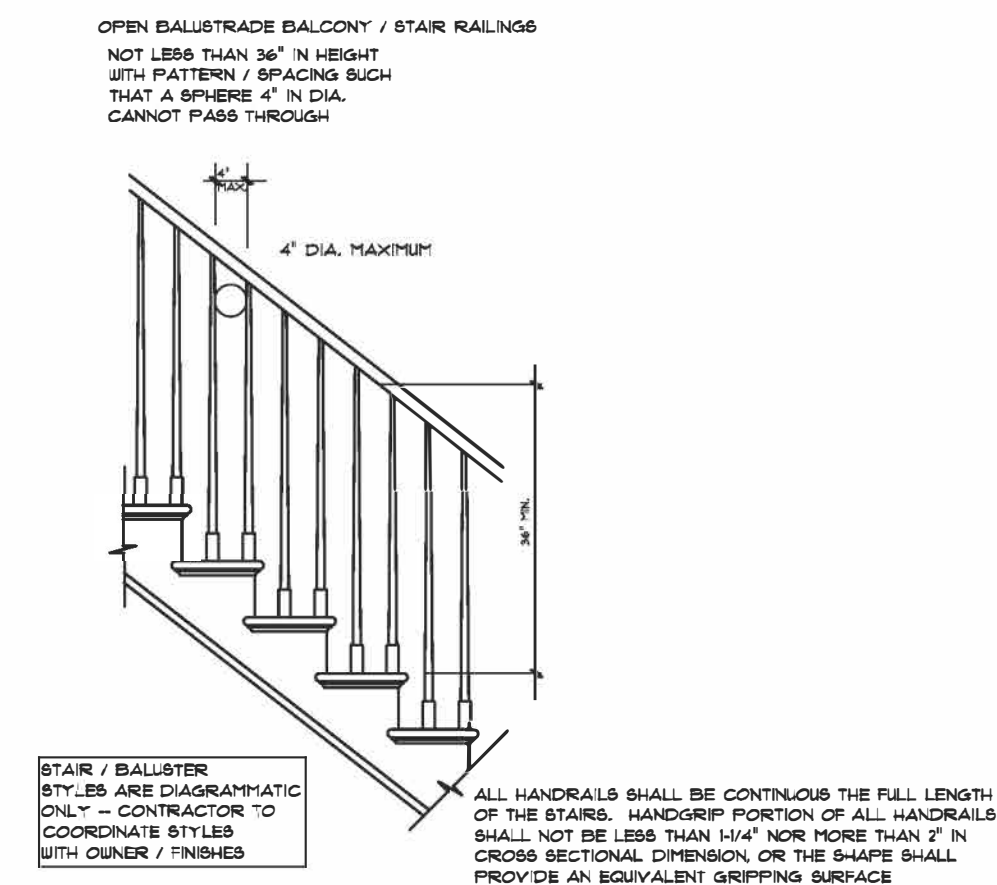
STAIR RAILING DETAIL/NOTES
