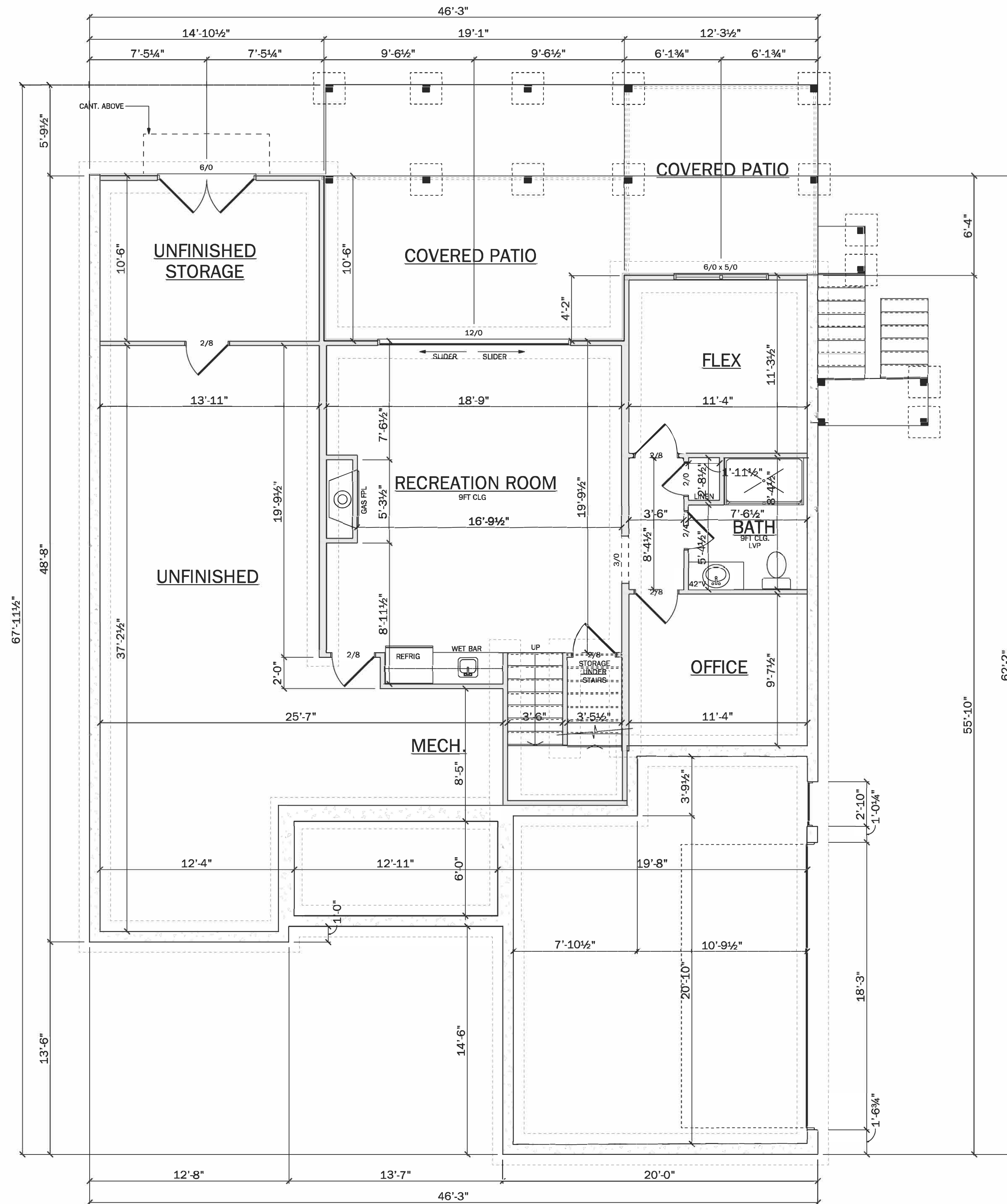
BASEMENT SCALE: 1/4" = 1'-0"
