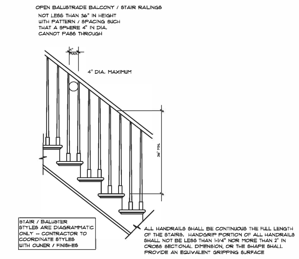
STAIR RAILING DETAIL/NOTES
