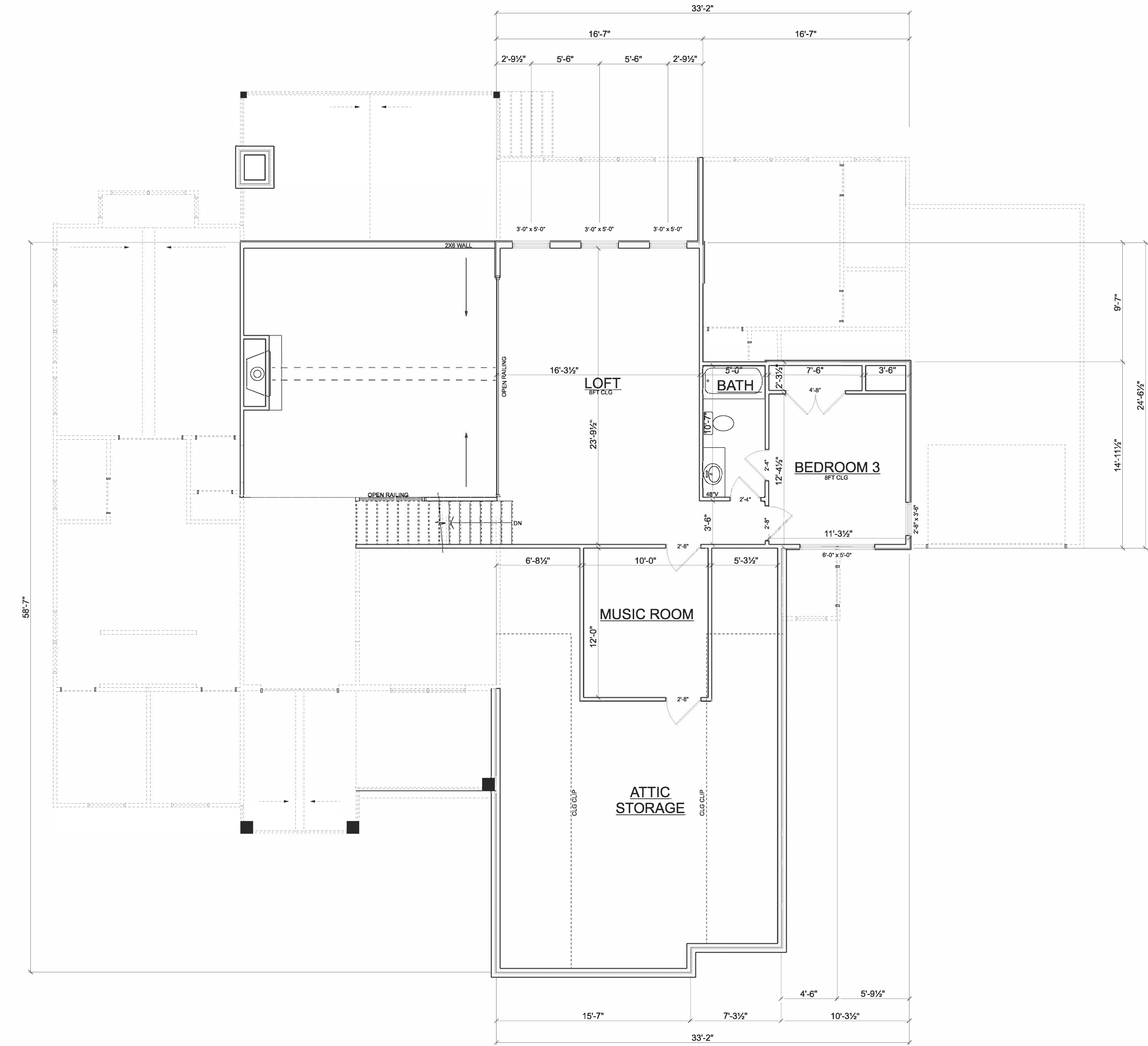
SECOND FLOOR SCALE: 1/4" = 1'-0"
